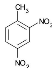
4. 2,4-Dinitrotoluene
